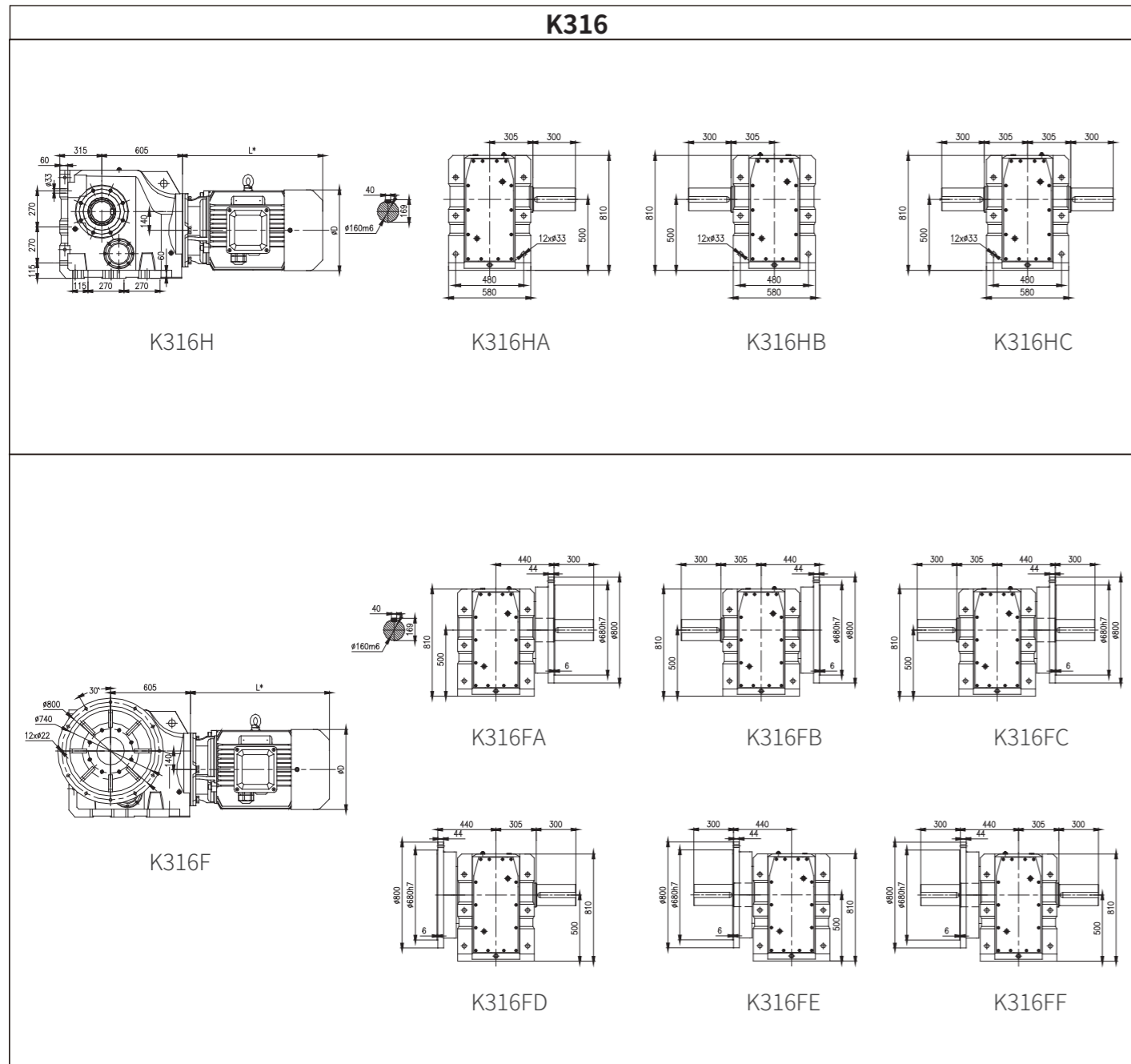
MP motor dimension for K316
