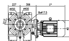
Flange-mounted (F) Weight: 250kg (Without motor and oil)
