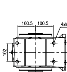
Torque arm-mounted without accessory (A) Weight: 45kg (Without motor and oil)
