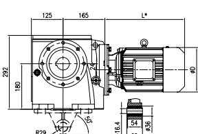
Torque arm-mounted with accessory (T) Weight: 50kg (Without motor and oil)
