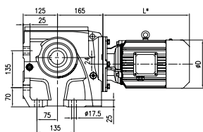
Horizontal foot-mounted (H) Weight: 45kg (Without motor and oil)
