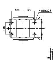
Torque arm-mounted without accessory (A) Weight: 85kg (Without motor and oil)
