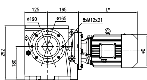
Short flange-mounted (S) Weight: 45kg (Without motor and oil)
