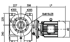
Short flange-mounted (S) Weight: 235kg (Without motor and oil)
