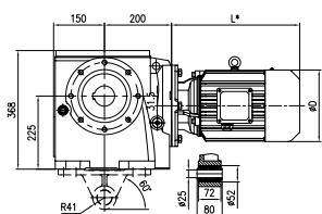
Torque arm-mounted with accessory (T) Weight: 95kg (Without motor and oil)
